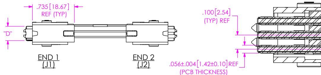
SECTION "A"- "A" SCALE 2.5 : 1
