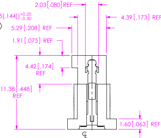
FIG 1 ISD2-05-D-M SHOWN
