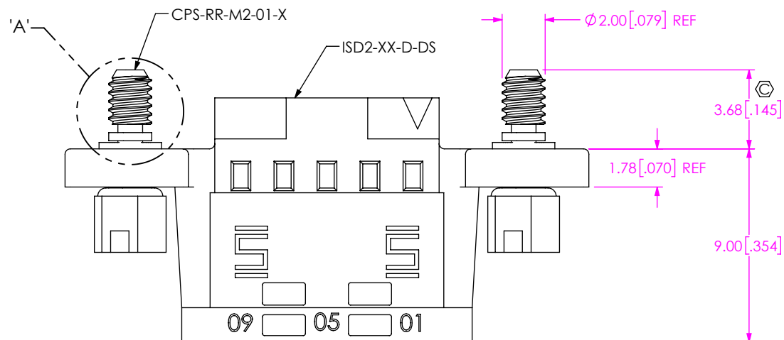
FIG 2 -S: DUAL SCREW DOWN OPTION ISD2-05-D-S SHOWN (DIFFERENT AS SHOWN, OTHERWISE SAME AS FIG 1)
