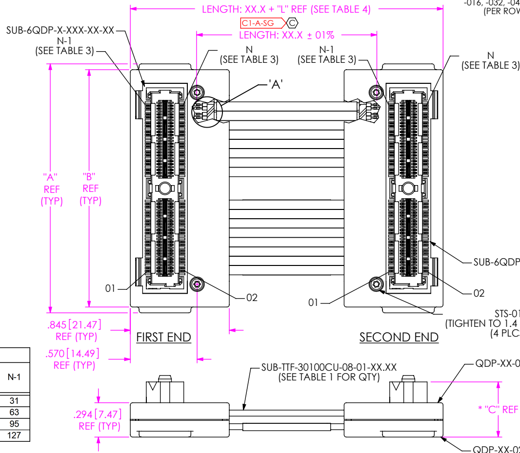
FIG 1 VERTICAL (6QDP-032-XX.X-STR-5 SHOWN)
