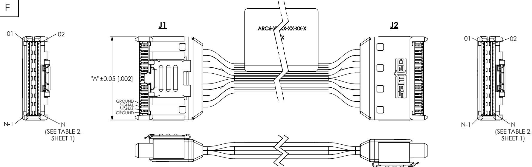
FIG 2 ARC6-16-XX.X-LU-LD-2-X SHOWN (DIFFERENT AS SHOWN, OTHERWISE SAME AS FIG 1)
