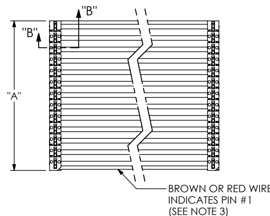
FIG 2 XDMS-13-D-XX.XX-X-X-X SHOWN (DIFFERENT AS SHOWN, OTHERWISE SAME AS FIG 1)
