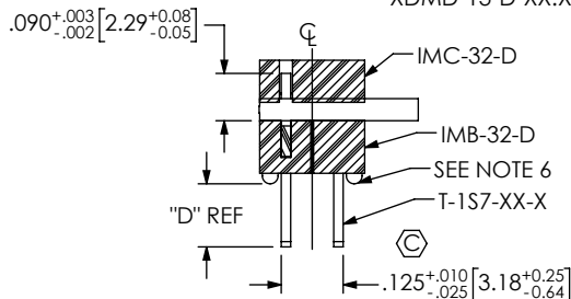
SECTION "A"-"A" (XDMD ASSEMBLY) (REFER TO XDM-XX-X ASSEMBLY)
