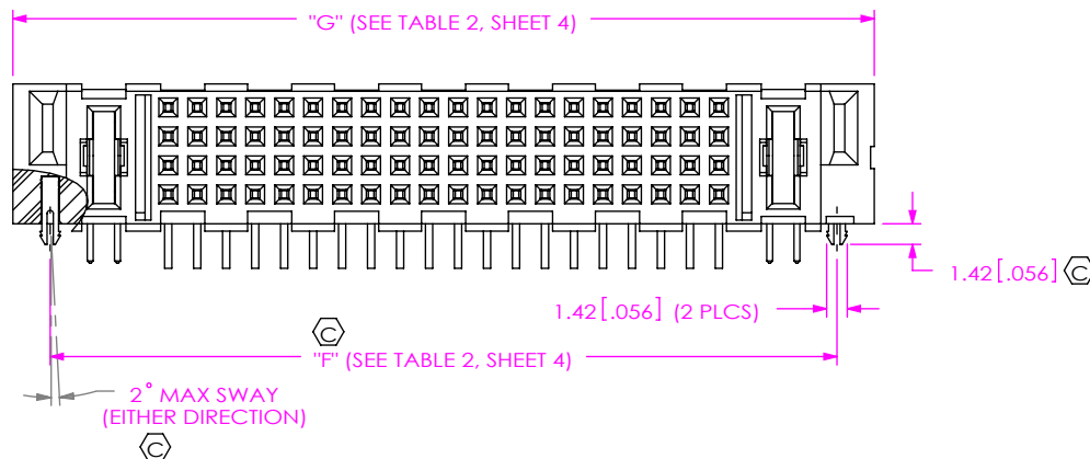
FIG 2 MPSC-01-80-01-01-X-RA-LC SHOWN (SAME AS FIG 1, UNLESS OTHERWISE STATED)
