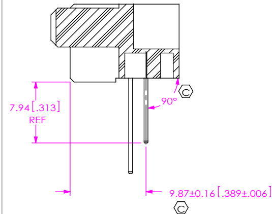
IN-PROCESS 4 BEND ROW 2
