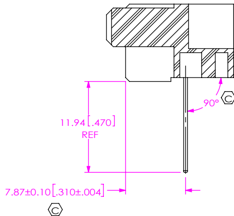
IN-PROCESS 2 BEND ROW 1
