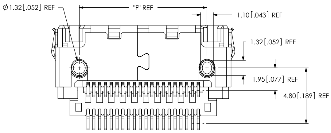
FIG 2 (SHIELD OPTION) LSHM-1XX-X1-XX-DH-A-S-XX-XX SHOWN
