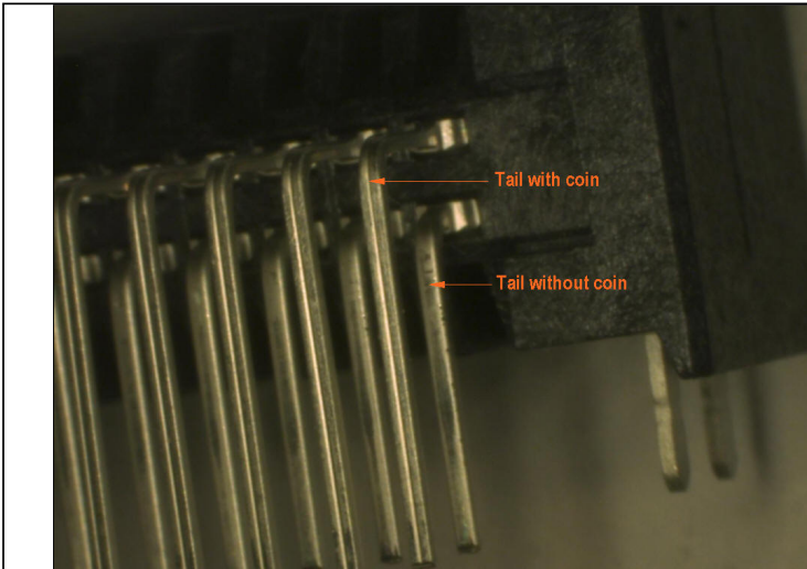
TFM ASSEMBLY WITH "TAIL WITH" AND "TAIL WITHOUT" COIN
