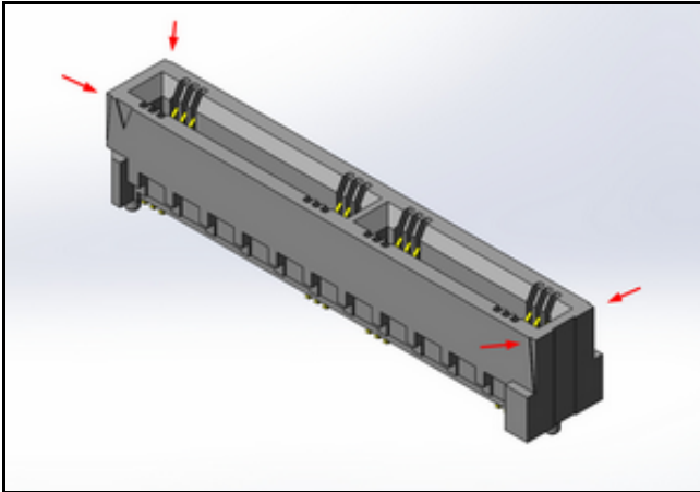
HSEC8 Connector with corner voids (4 plcs)
