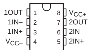
TL062, TL062A, TL062B D, JG, P, OR PW PACKAGE (TOP VIEW)
