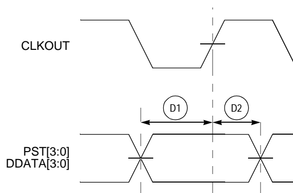
Figure 32-16. Real-Time Trace AC Timing
