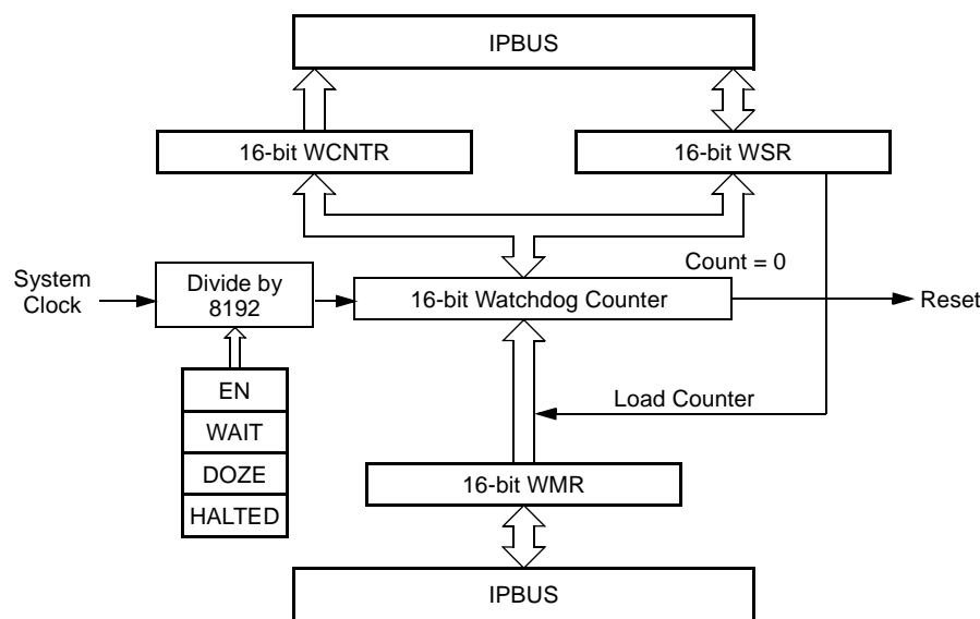
Figure 17-1. Watchdog Timer Block Diagram
