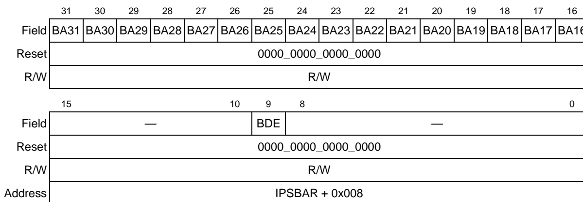
Figure 8-2. Memory Base Address Register (RAMBAR)
