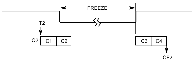
Figure 26-35. CCW Freeze Situation 13
