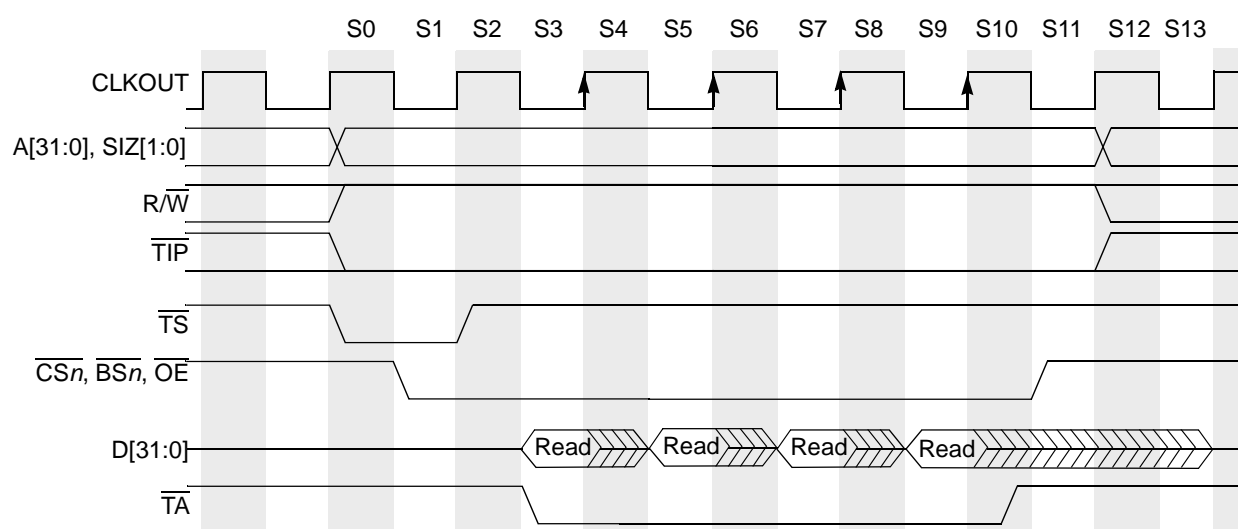
Figure 13-12. Line Read Burst (2-1-1-1), External Termination
