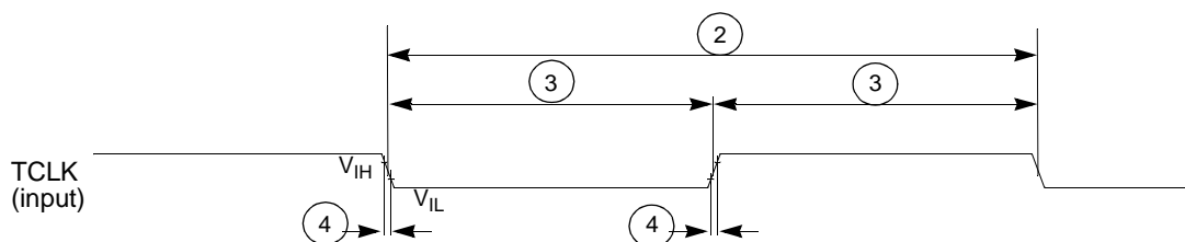
Figure 32-11. Test Clock Input Timing
