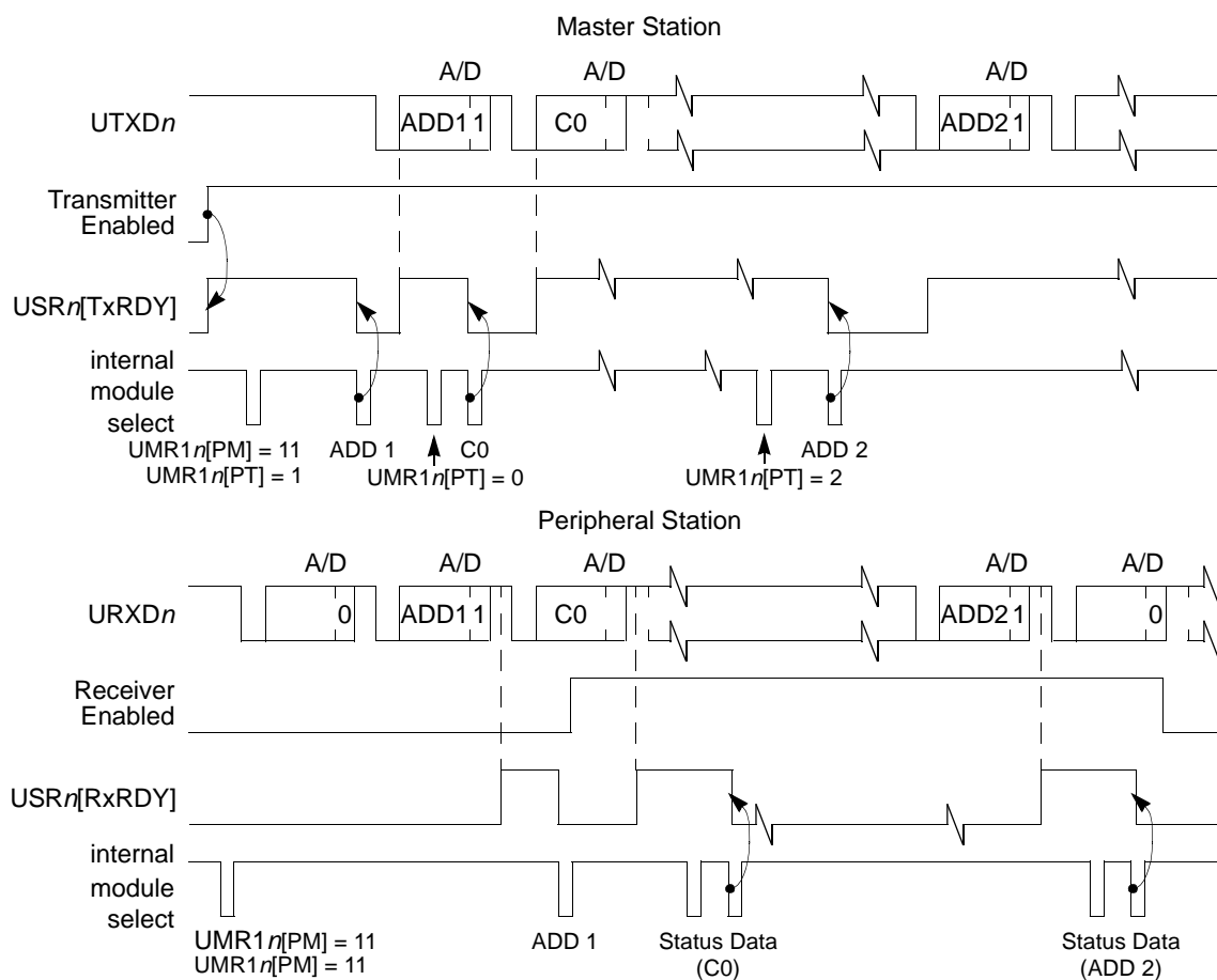
Figure 22-25. Multidrop Mode Timing Diagram
