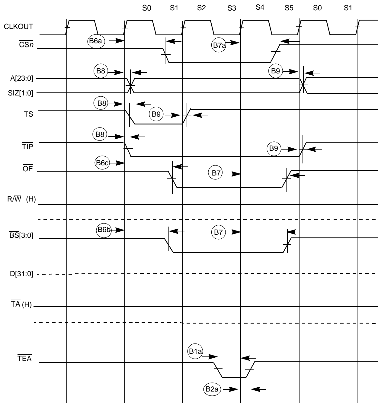
Figure 32-4. Read Bus Cycle Terminated by \overline{TEA}
