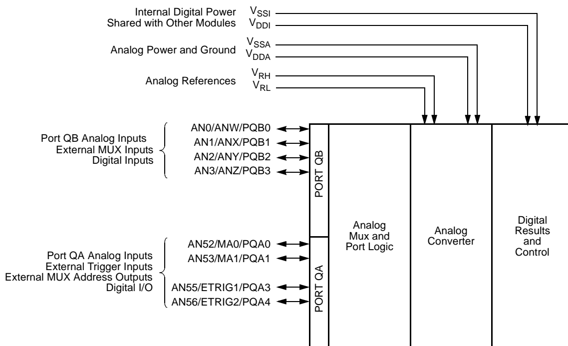
Figure 26-2. QADC Input and Output Signals
