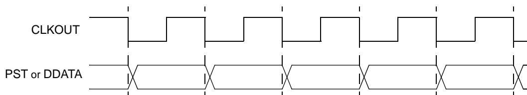
Figure 28-2. CLKOUT Timing
