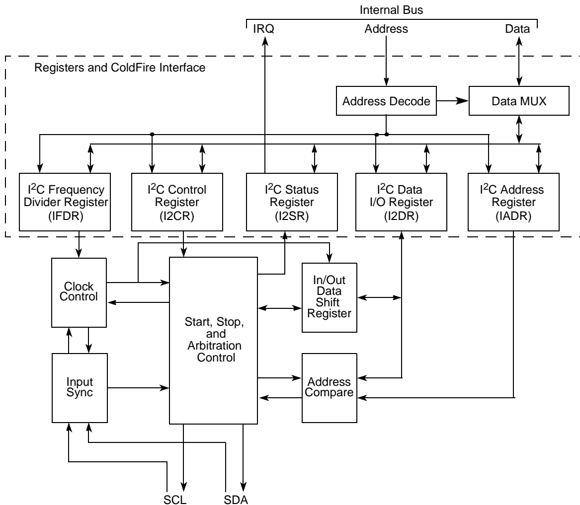
Figure 23-1. I 2 C Module Block Diagram
