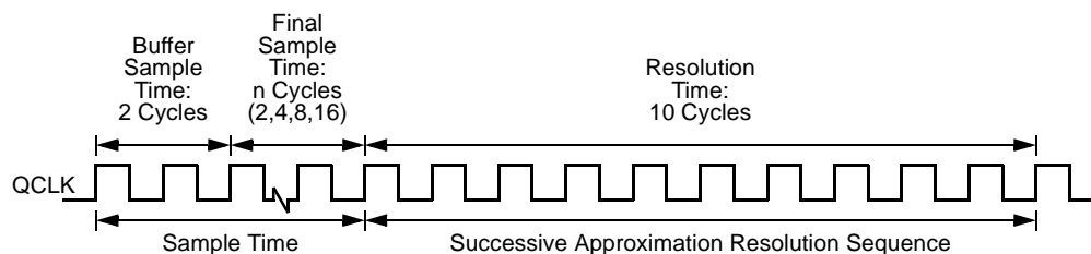
Figure 26-20. Conversion Timing
