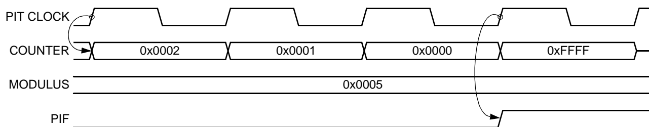
Figure 18-6. Counter in Free-Running Mode
