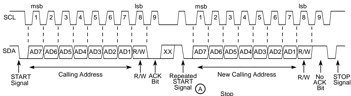
Figure 23-3. Repeated START
