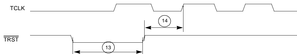
Figure 32-14. TRST Timing
