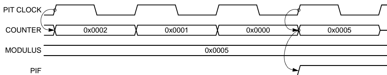
Figure 18-5. Counter Reloading from the Modulus Latch
