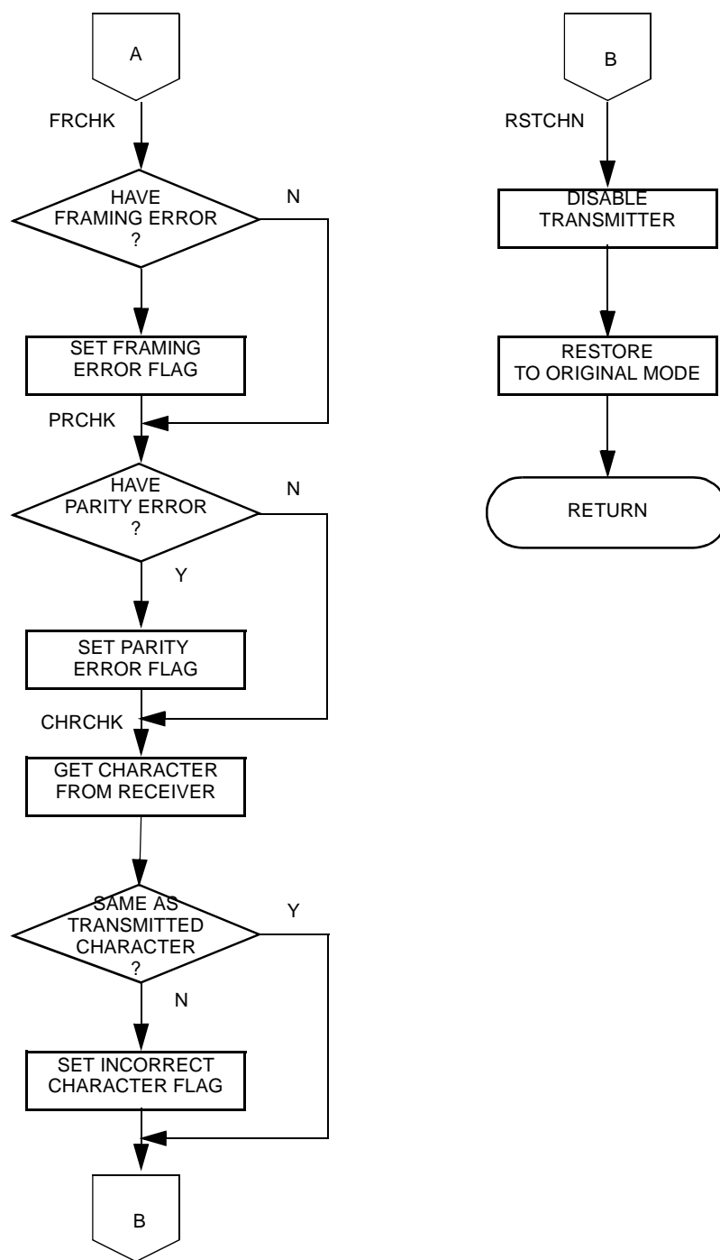
Figure 22-26. UART Mode Programming Flowchart (Sheet 3 of 5)
