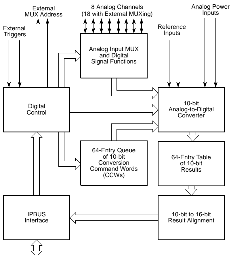
Figure 26-1. QADC Block Diagram
