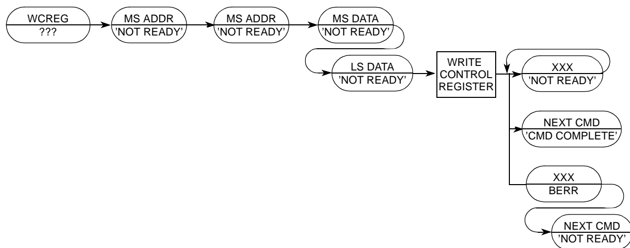
Figure 28-36. WCREG Command Sequence
