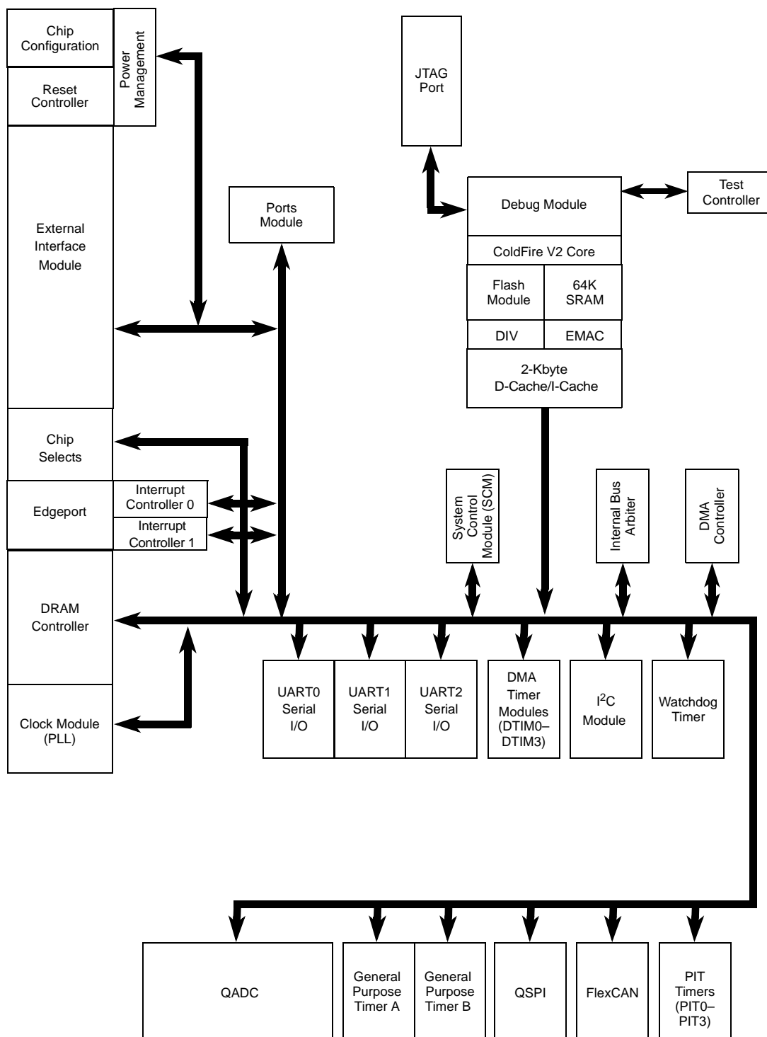
Figure 1-1. MCF5216 Block Diagram
