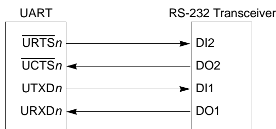
Figure 22-17. UART/RS-232 Interface
