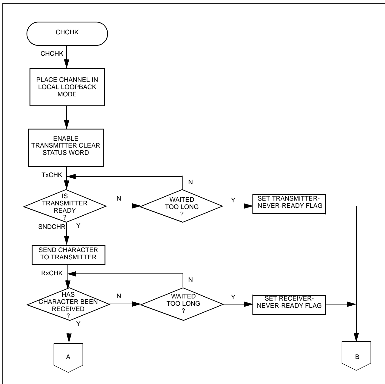
Figure 22-26. UART Mode Programming Flowchart (Sheet 2 of 5)
