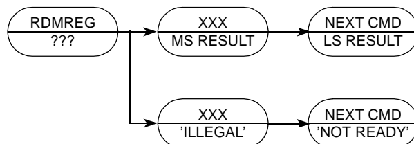
Figure 28-38. RDMREG Command Sequence
