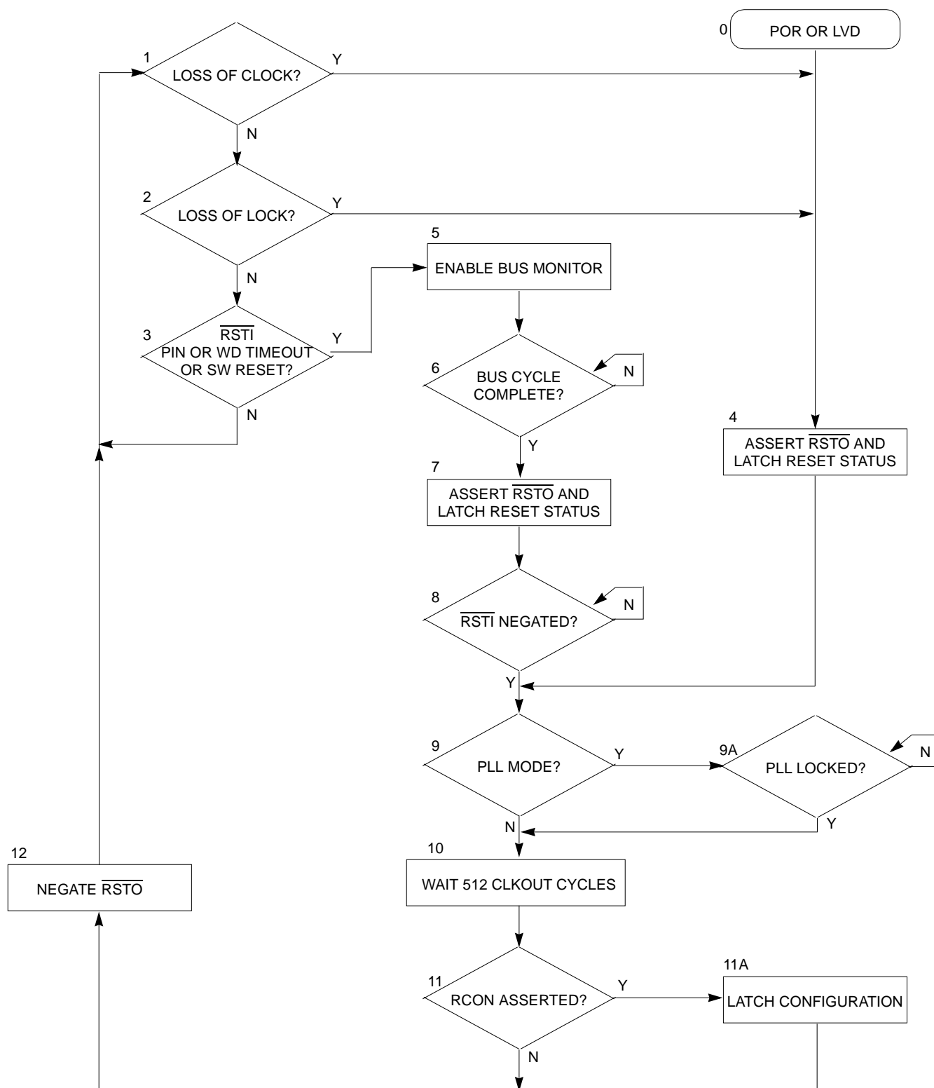
Figure 27-4. Reset Control Flow
