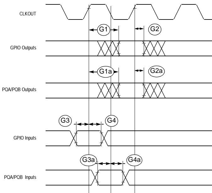
Figure 32-7. GPIO Timing
