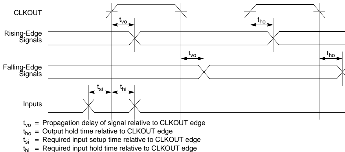
Figure 13-1. Signal Relationship to CLKOUT for Non-DRAM Access
