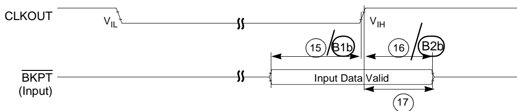
Figure 32-15. \overline{\text{BKPT}} Timing
