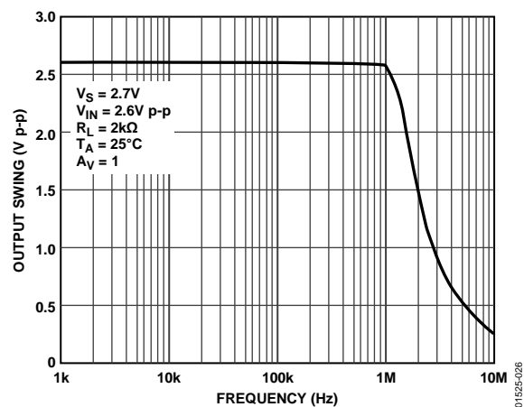
Figure 26. Closed-Loop Output Voltage Swing vs. Frequency
