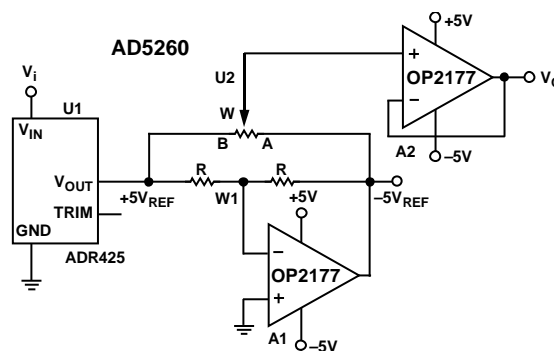
Figure 61. 8-Bit Bipolar DAC
