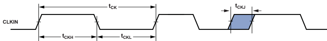
Figure 7. Clock Input
