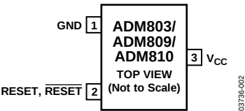
Figure 3. Pin Configuration
