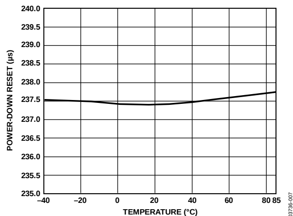
Figure 7. Power-Down RESET Delay vs. Temperature ADM8_R
