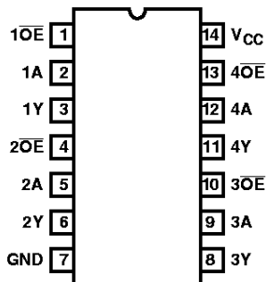
CD74HC125, CD74HCT125 (PDIP, SOIC) TOP VIEW
