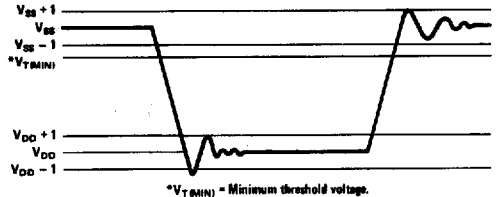
FIGURE 3. Clock Waveform
