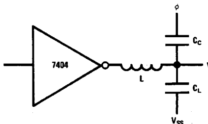
FIGURE 5. Clock Coupling
