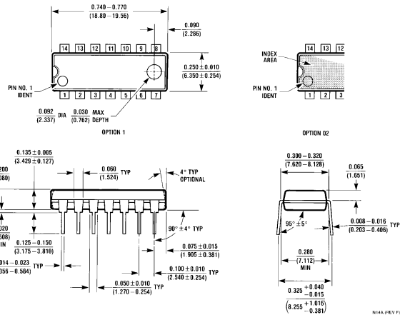
Molded Dual-In-Line Package (N) Order Number MM74HC164N NS Package Number N14A
