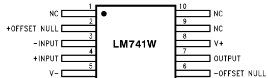
Ceramic Flatpak
