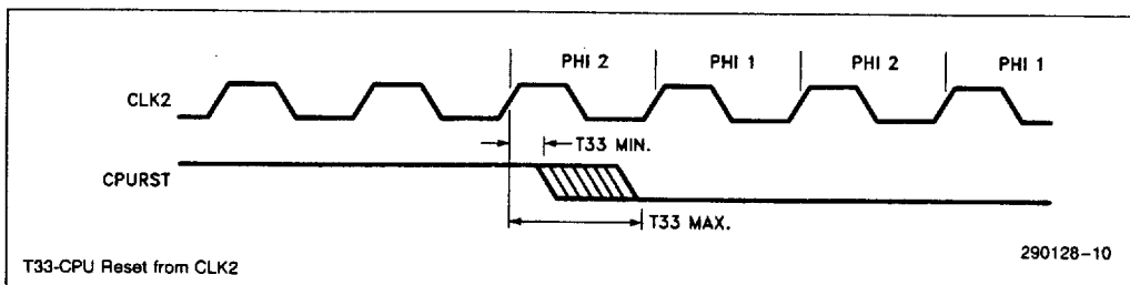
Figure 2-4. CPURST Timing
