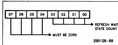
REFRESH WAIT STATE REGISTER
