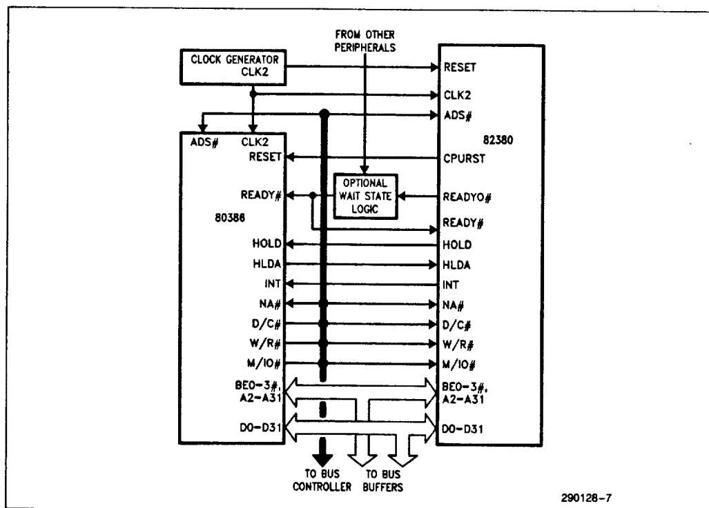
Figure 2-1. 80386/82380 System Configuration
