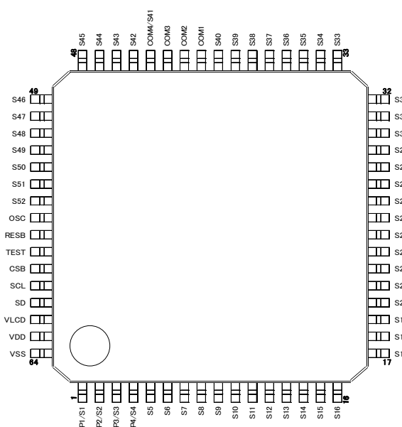
Figure 3. Pin Configuration (TOP VIEW)
