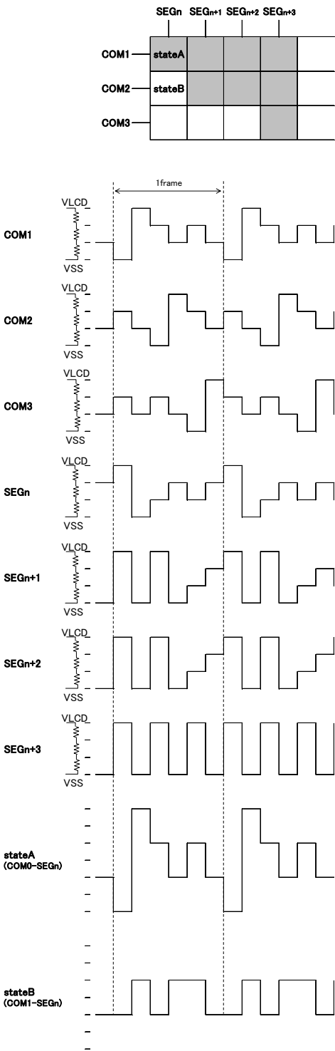
Figure 15. LCD waveform in line inversion
