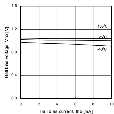
Fig.3 Hall bias voltage
