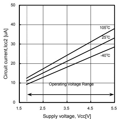
Fig.2 Circuit current 2
