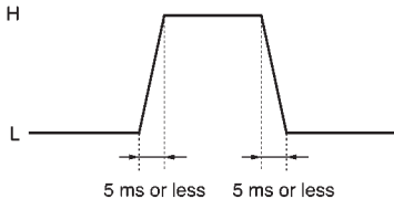
Fig.17 Control signal
