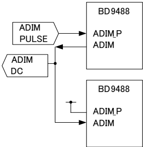
Figure 13. the analog dimming circuit as two BD9488 are used.
