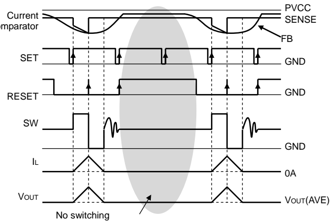
Figure.29 SLLM™ Switching timing chart
