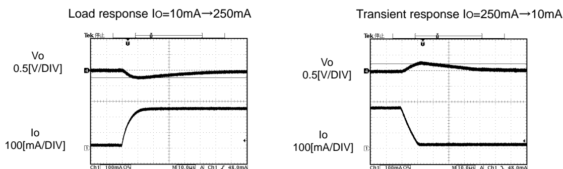
Figure.25 Transient response
