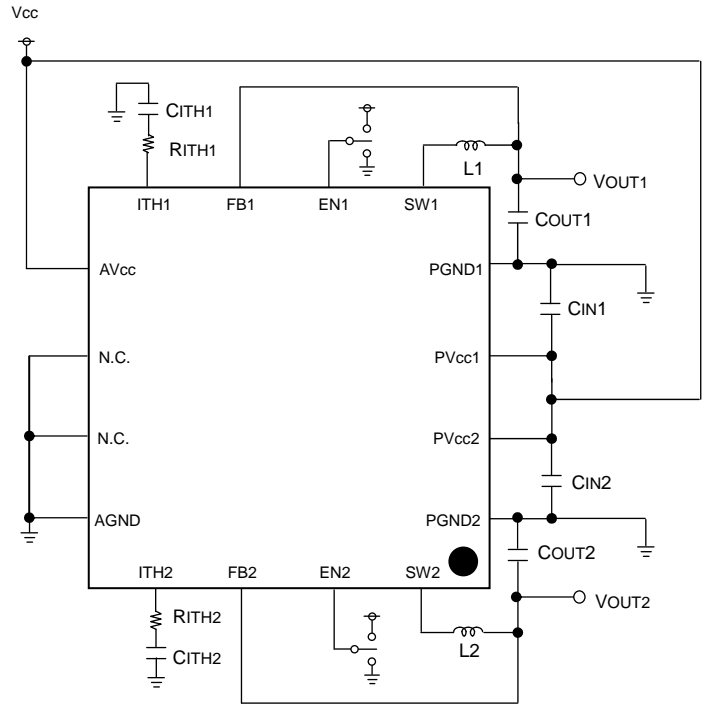
Figure.38 Application Example
