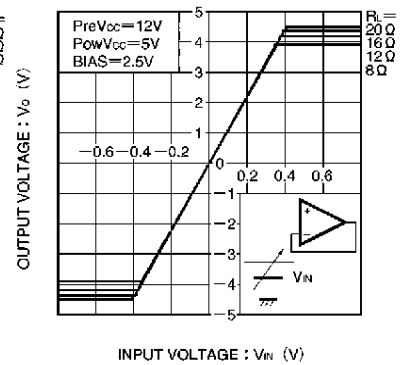
Fig. 13 Driver I/O characteristics (sled)
