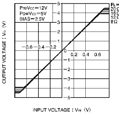
Fig. 14 Driver I/O characteristics (loading)
