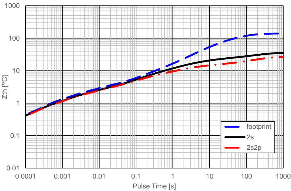
Figure 5. Transient Thermal Resistance
