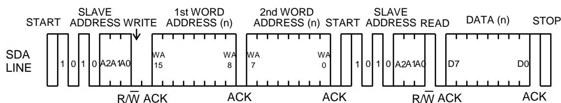
Figure 44. Random Read
