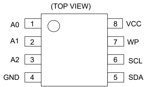
Figure 3. Pin Configuration
