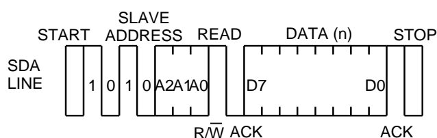
Figure 45. Current Read
