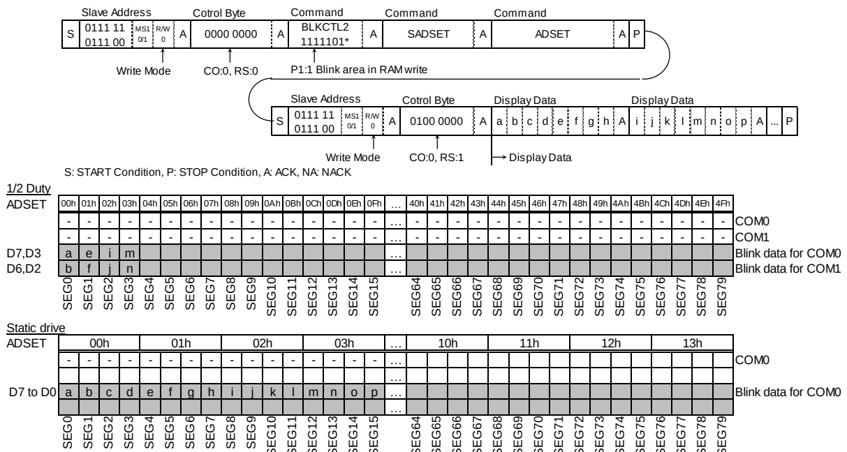
Figure 31. DDRAM Address Map of Blink Area (Bank Blink Mode)
