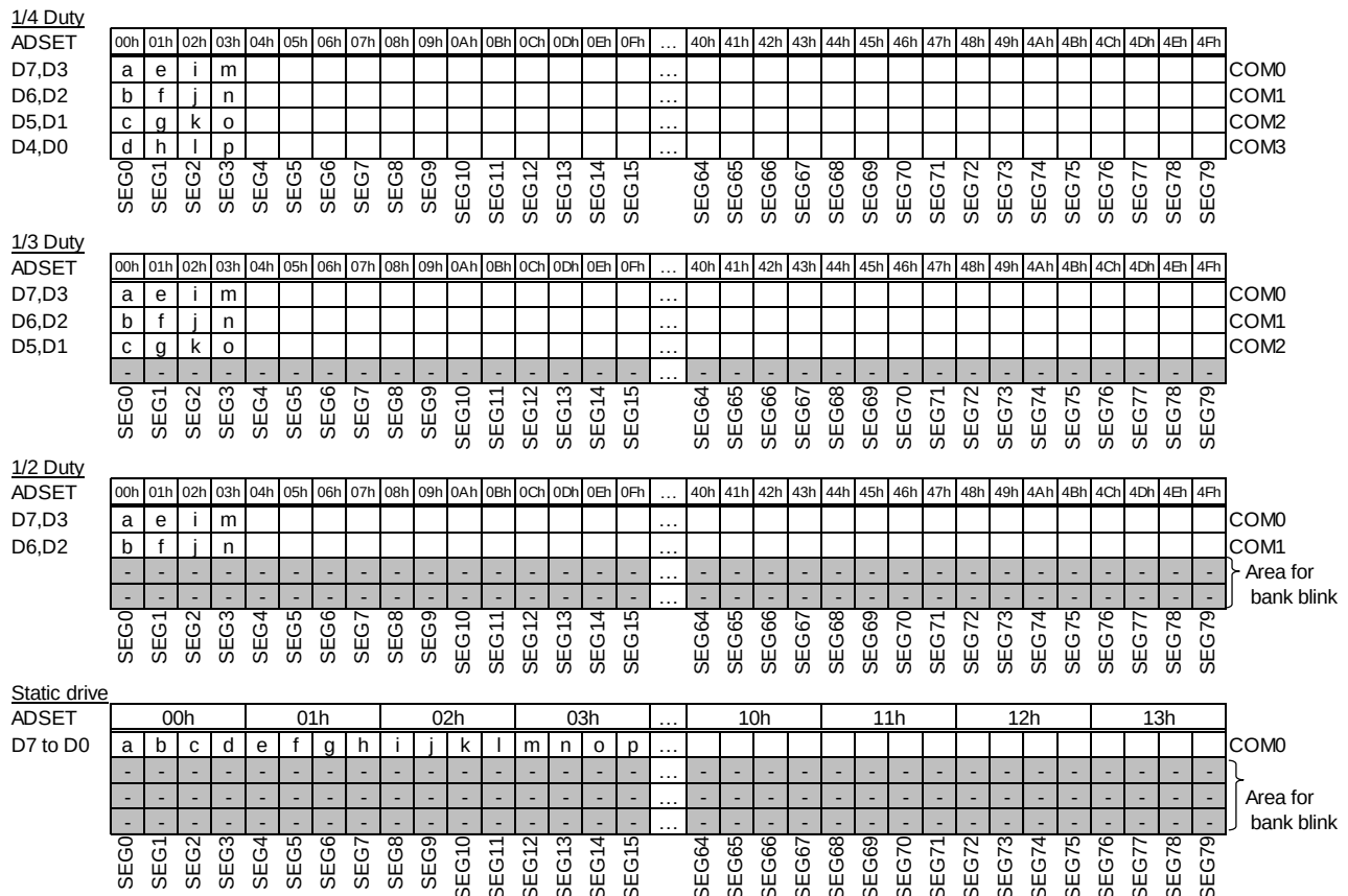
Figure 12. DDRAM Address Map in Write Mode
