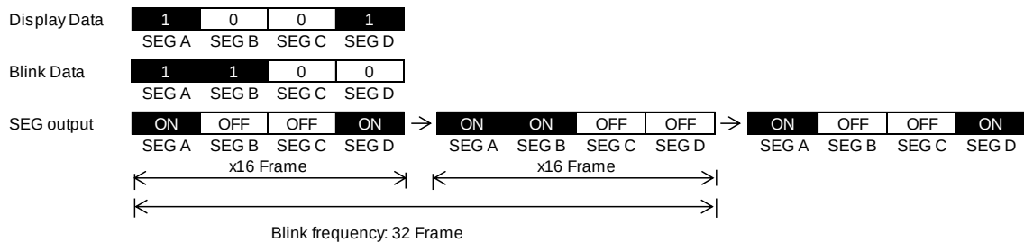
Figure 30. Bank Blink Mode Function (Blink Frequency as 32 Frame Case)
