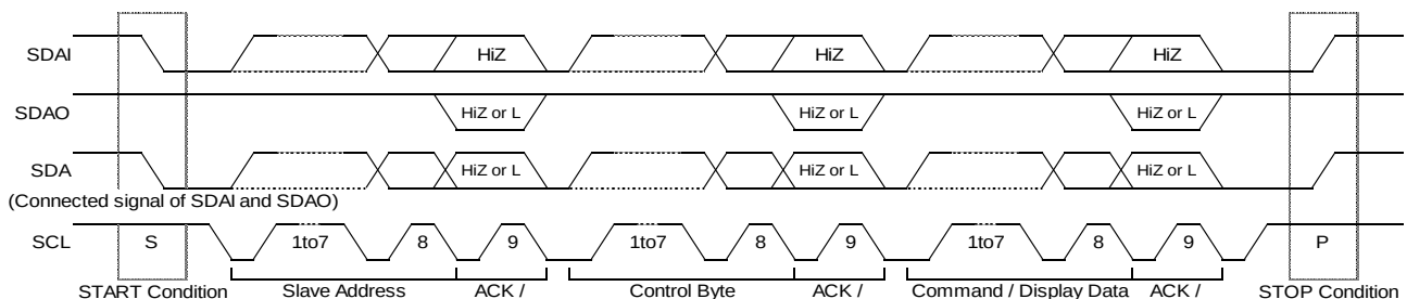
Figure 7. Acknowledge Timing
