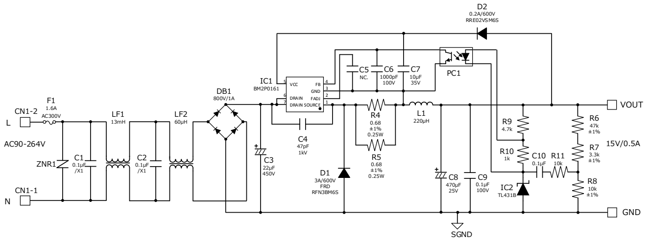
Figure 3. BM2P0161-EVK-001 Schematics
