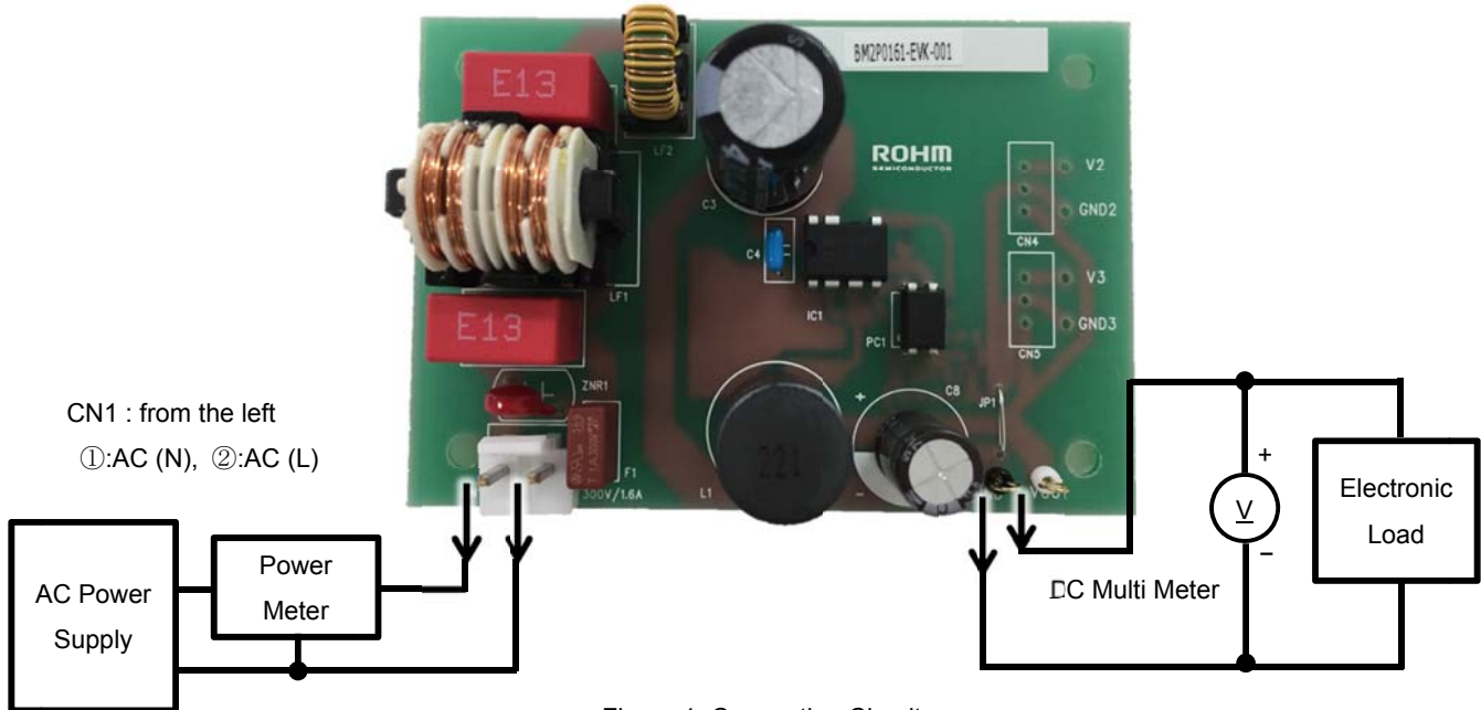
Figure 1. Connection Circuit
