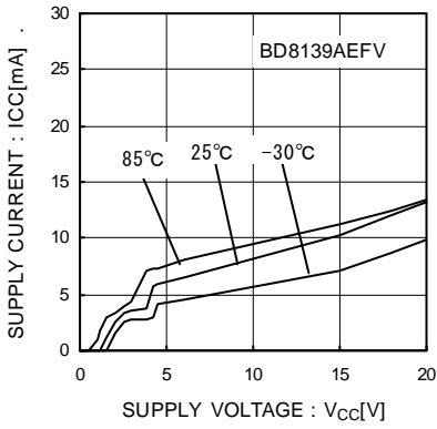
Fig. 4 Vcc Total Supply Current
