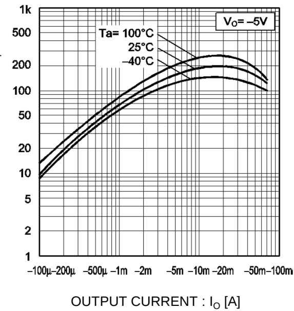
Fig.9 DC current gain vs. output current
