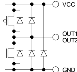
Figure 46. OUT1 / OUT2 (SOP8/HRP7)
