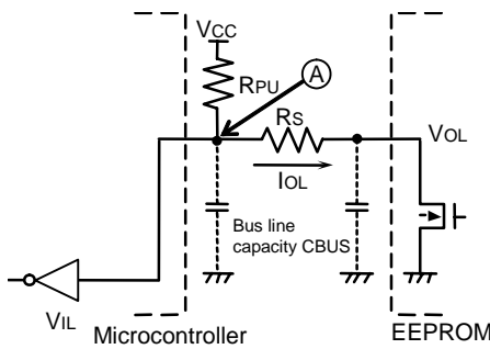
Figure 54. I/O circuit
