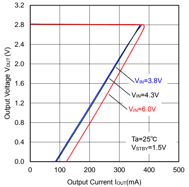
Figure 29. OCP Threshold
