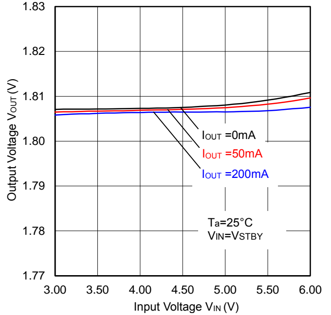
Figure 4. Line Regulation
