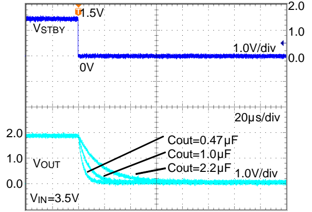
Figure 23. Discharge Time (ROUT=9Ω)
