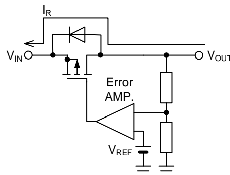
Figure 51. Reverse Current Path in an MOS Linear Regulator
