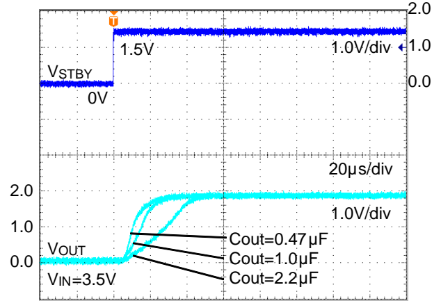
Figure 21. Startup Time (ROUT=9Ω)
