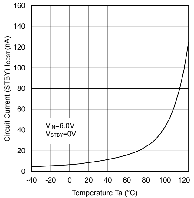
Figure 33. Circuit Current (STBY) vs. Temperature
