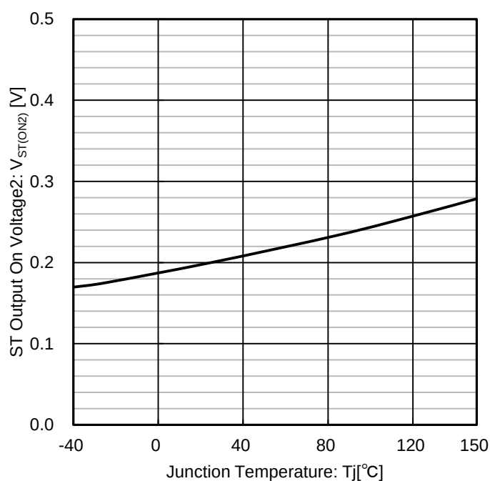
Figure 26. ST Output On Voltage2 vs. junction temperature
