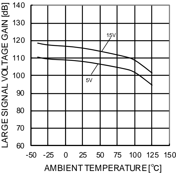
Figure 94. Large Signal Voltage Gain - Ambient Temperature ( R_L=2k\Omega )
