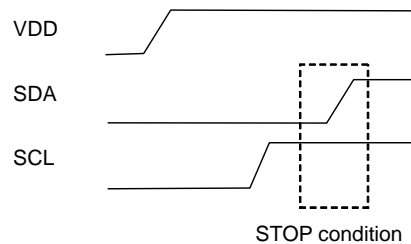
Figure 23. STOP Condition
