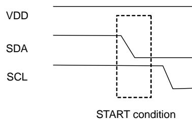
Figure 24. START Condition
