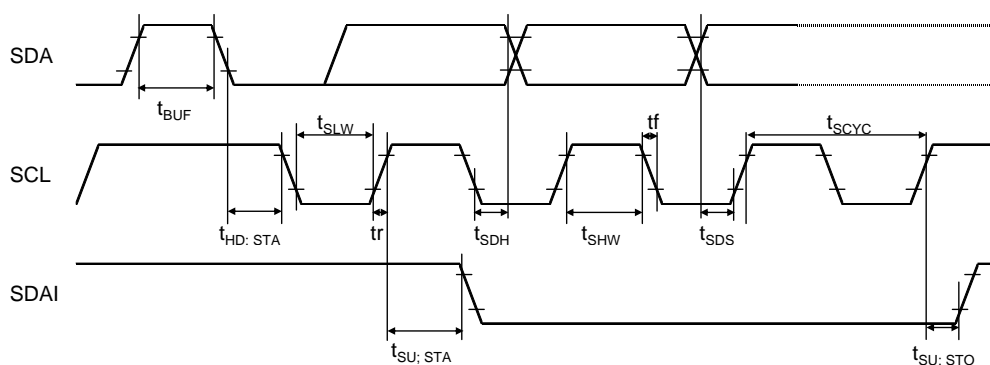
Figure 7. Interface Timing
