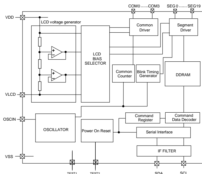
Figure 4. Block Diagram
