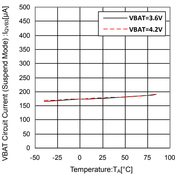
Figure 25. VBAT Circuit Current (Suspend Mode) vs Temperature
