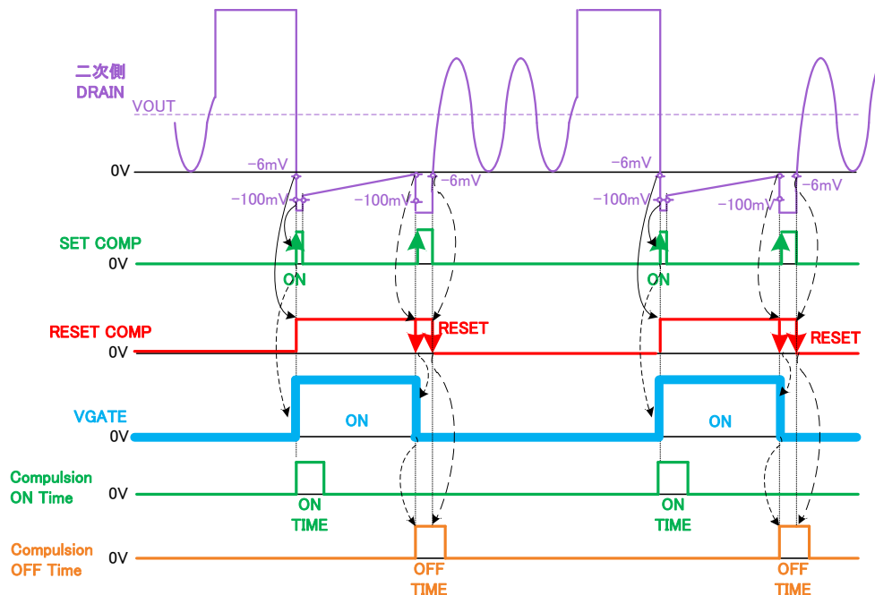
Figure 1. Operation sequence
