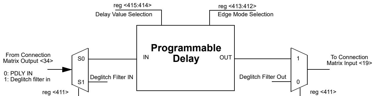
Figure 23. Programmable Delay
