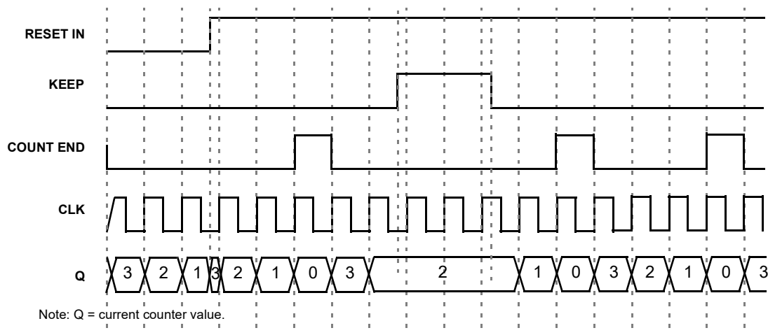
Figure 20. Timing (Set Rising Edge Mode, Oscillator is Forced On, UP = 0) for Count Data = 3
