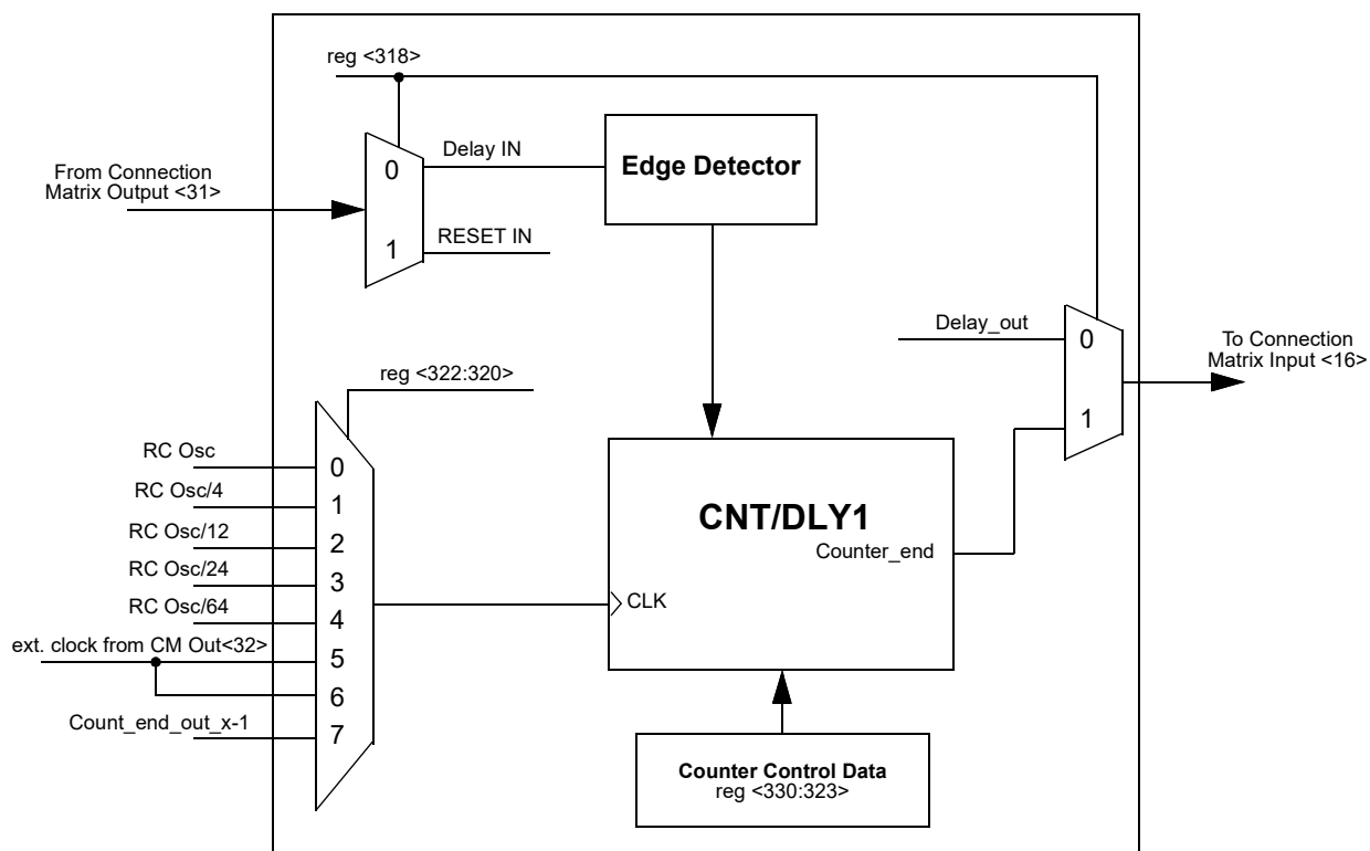
Figure 27. CNT/DLY1
