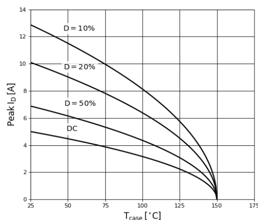
Figure 13. Current Derating
