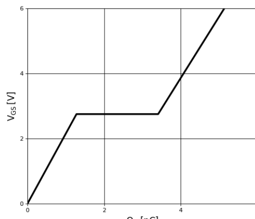
Figure 11. Typical Gate Charge
