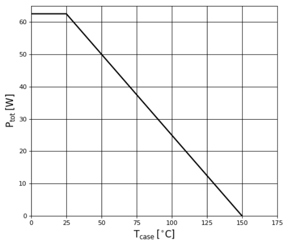
Figure 12. Power Dissipation
