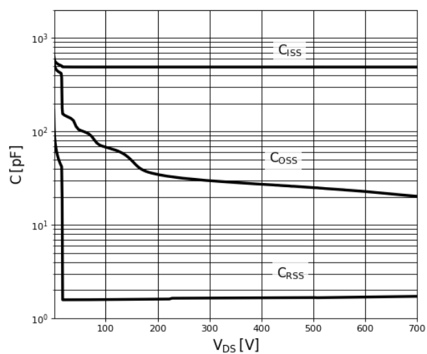
Figure 8. Typical Capacitance
