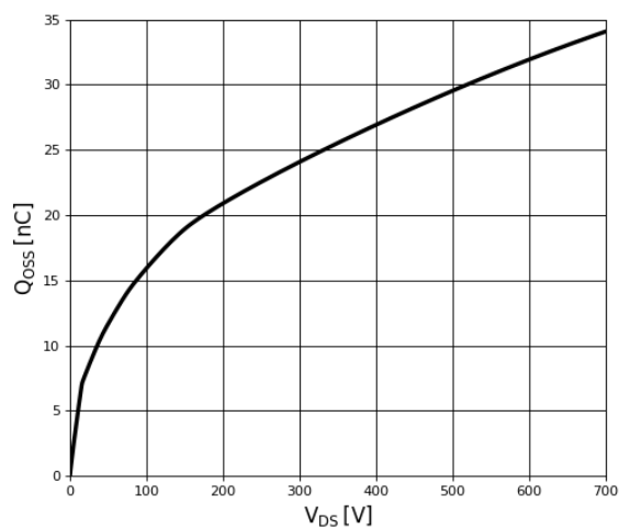
Figure 10. Typical Q_{oss}
