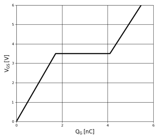
Figure 11. Typical Gate Charge
