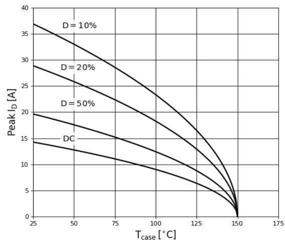
Figure 13. Current Derating Pulse width \leq 10\mu\text{s} , V_{GS} \geq 6\text{V}
