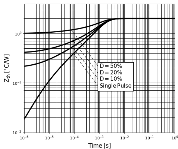
Figure 15. Transient Thermal Resistance
