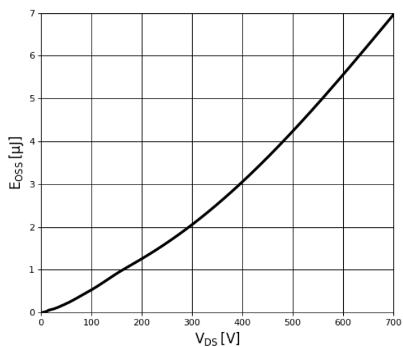
Figure 9. Typical C_{oss} Stored Energy
