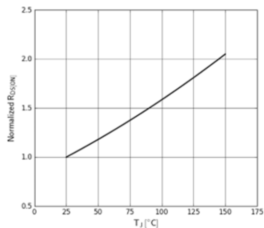
Figure 7. Normalized On-resistance I_D = 10\text{A} , V_{GS} = 6\text{V}
