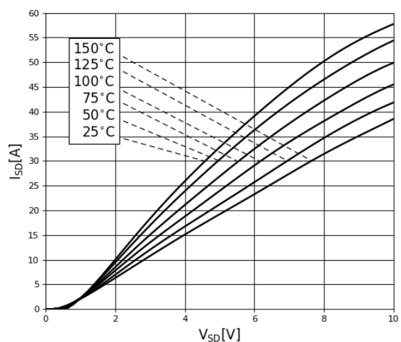
Figure 14. Forward Characteristics of Rev. Diode I_S = f(V_{SD}) , parameter: T_J
