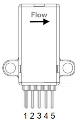
Figure 2. Pin Assignments
