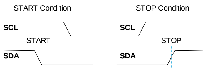
Figure 6. START and STOP Condition Waveform
