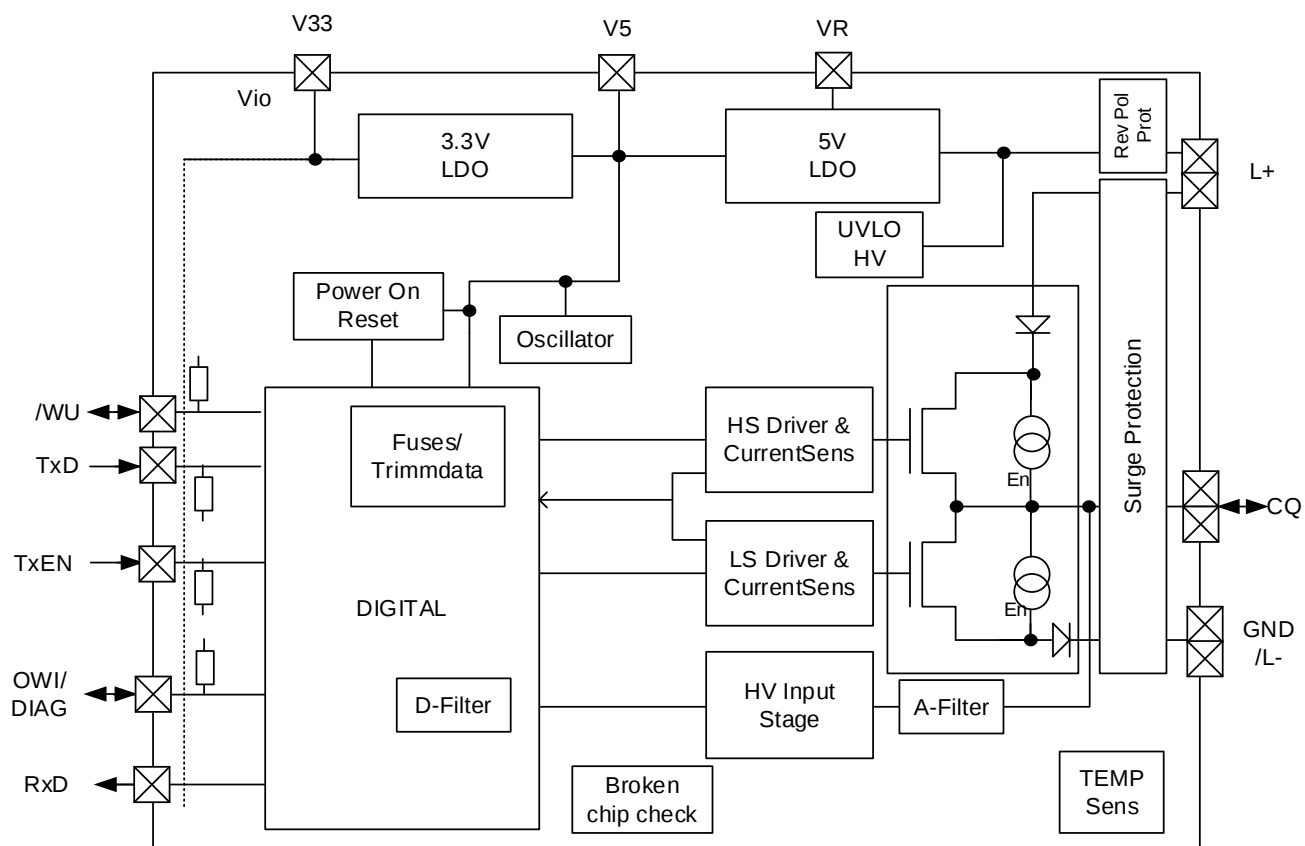
Figure 2. Block Diagram
