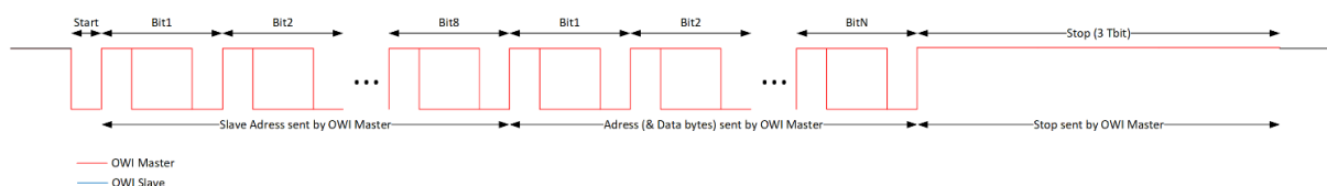
Figure 23: OWI Write Command Chronogram
