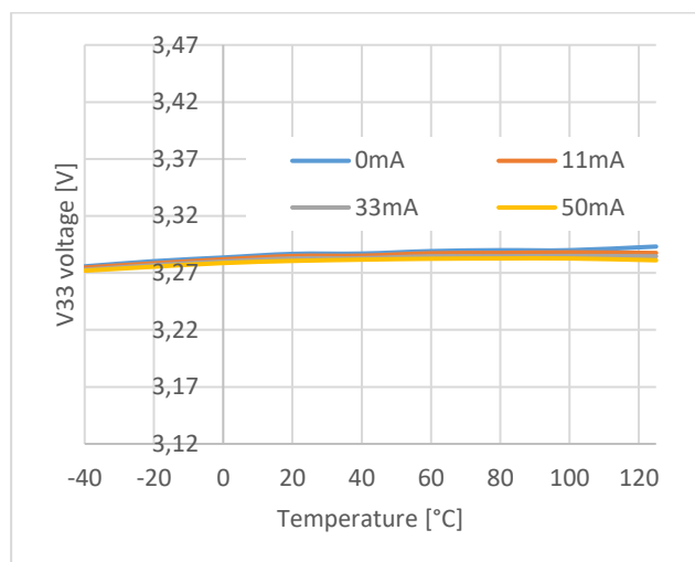
Figure 16. V33 Output Voltage vs. Temperature
