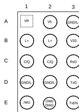
Figure 4. WCSP15 Pin Layout (Top View)
