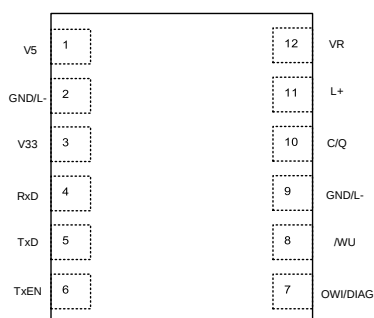
Figure 3. DFN 12 Pin Layout (Top View)
