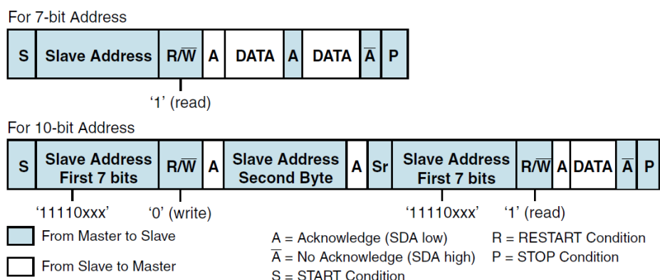
Figure 31: Master-Receiver Protocol
