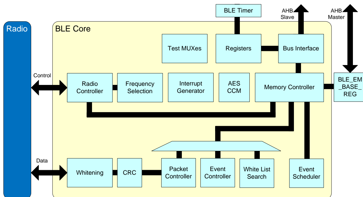
Figure 74: BLE Core Block Diagram
