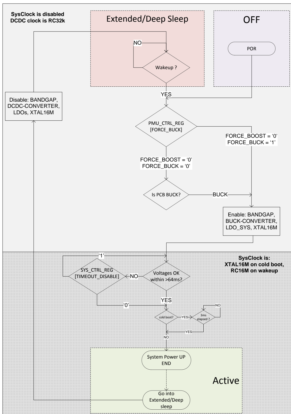
Figure 7: Power/Wake-Up Sequence
