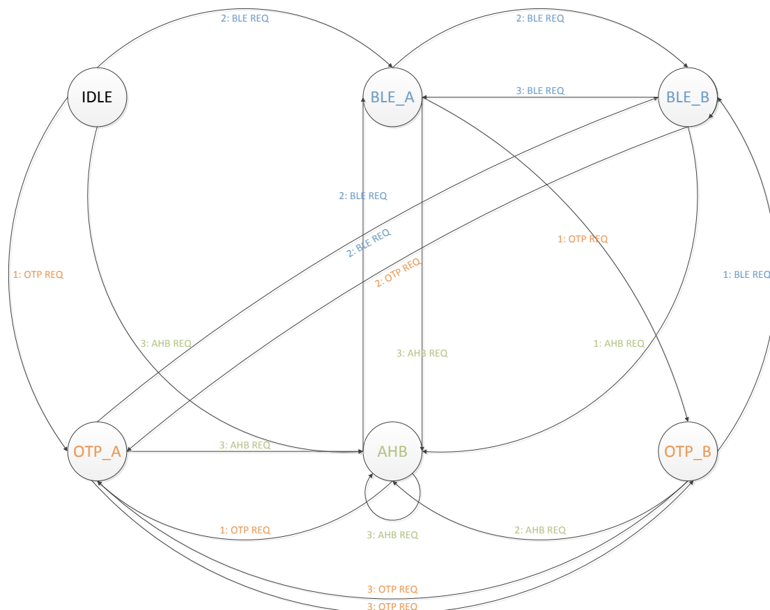
Figure 17: Arbitration Scheme
