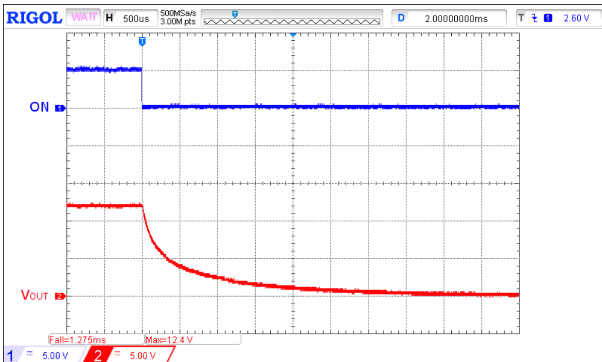
Figure 15. Typical Turn OFF operation waveform for V_{IN} = 12 V, C_{SLEW} = 10 nF, C_{LOAD} = 10 μF, R_{LOAD} = 100 Ω
