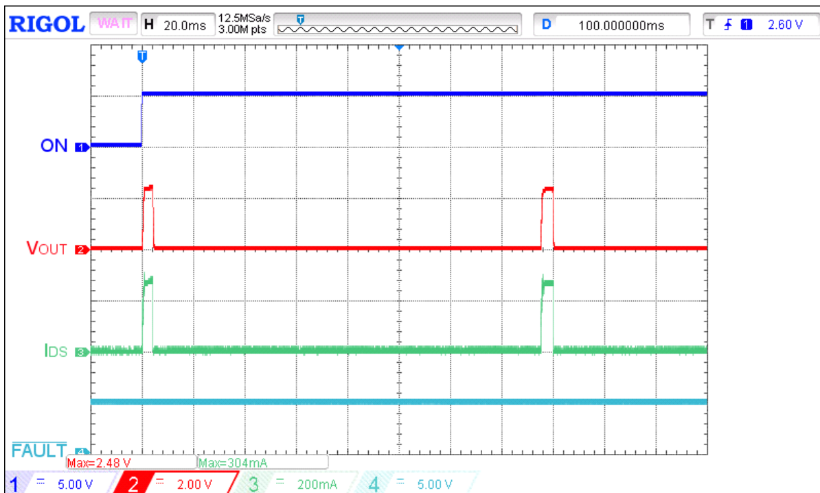
Figure 27. Extended typical SOA waveform during powerup on heavy load for V_{IN} = 20\text{ V} , C_{LOAD} = 10\text{ }\mu\text{F} , R_{SET} = 30.1\text{ k}\Omega , R_{LOAD} = 8\text{ }\Omega
