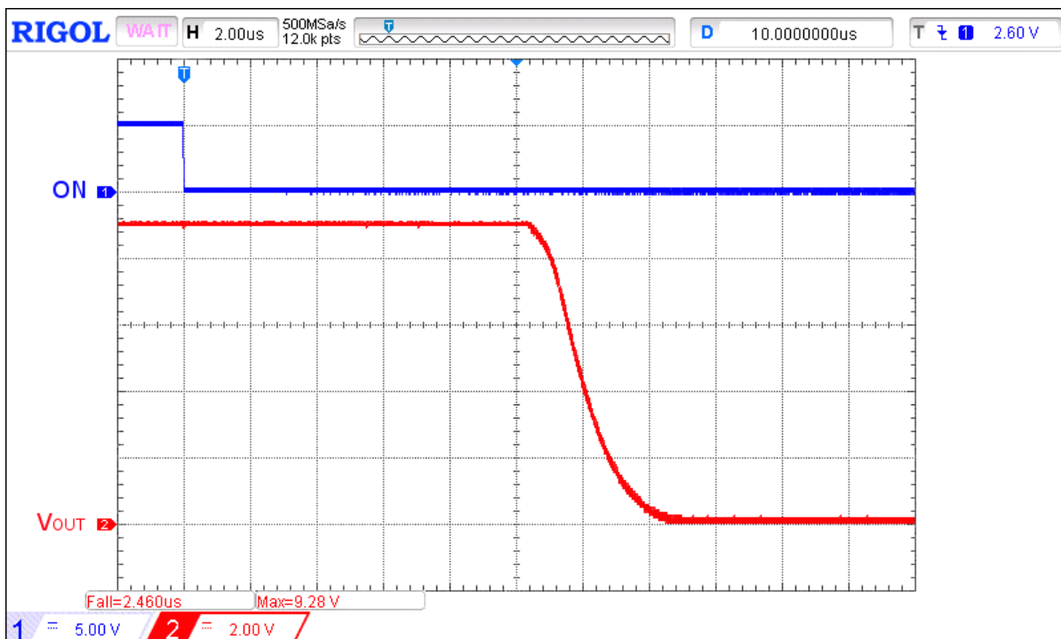
Figure 12. Typical Turn OFF operation waveform for V_{IN} = 9 V, C_{SLEW} = 10 nF, no C_{LOAD} , R_{LOAD} = 100 Ω
