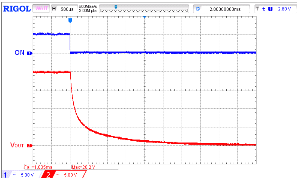
Figure 17. Typical Turn OFF operation waveform for V_{IN} = 20 V, C_{SLEW} = 10 nF, C_{LOAD} = 10 μF, R_{LOAD} = 100 Ω
