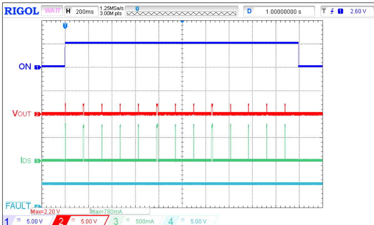
Figure 22. Typical SOA waveform during powerup on heavy load for V_{IN} = 9 V, C_{LOAD} = 10 \mu F, R_{SET} = 30.1 k \Omega , R_{LOAD} = 3.8 \Omega
