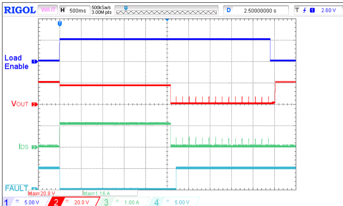
Figure 21. Thermally induced SOA shutdown for V_{IN} = 20 V, C_{LOAD} = 10 \mu F, I_{ACL} = 1 A, R_{SET} = 91 k \Omega
