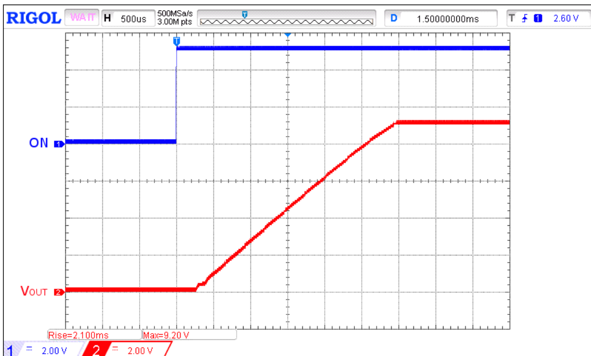
Figure 4. Typical Turn ON operation waveform for V_{IN} = 9 V, C_{SLEW} = 10 nF, C_{LOAD} = 10 μF, R_{LOAD} = 100 Ω
