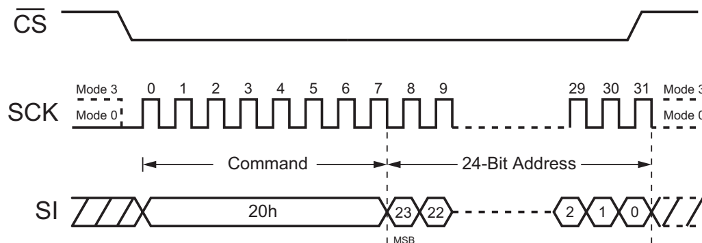
Figure 29. Block Erase Command (SPI Mode)
