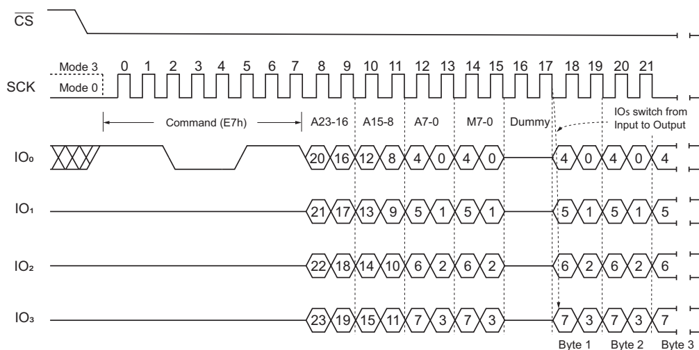
Figure 51. Word Read Quad I/O Command (Initial command or previous set M7-0 \neq Ah , SPI Mode)
