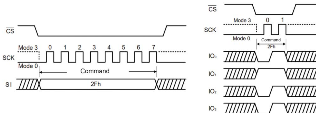
Figure 64. Write Security Register Command for SPI Mode (left) and QPI Mode (right)
