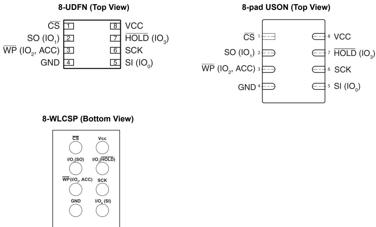
Figure 1. Package Types
