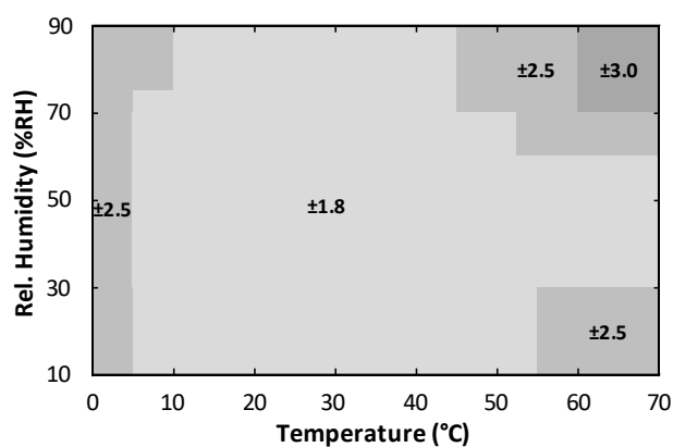
Figure 4. HS4112 RH Accuracy over Temperature
