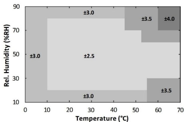
Figure 6. HS4113 RH Accuracy over Temperature
